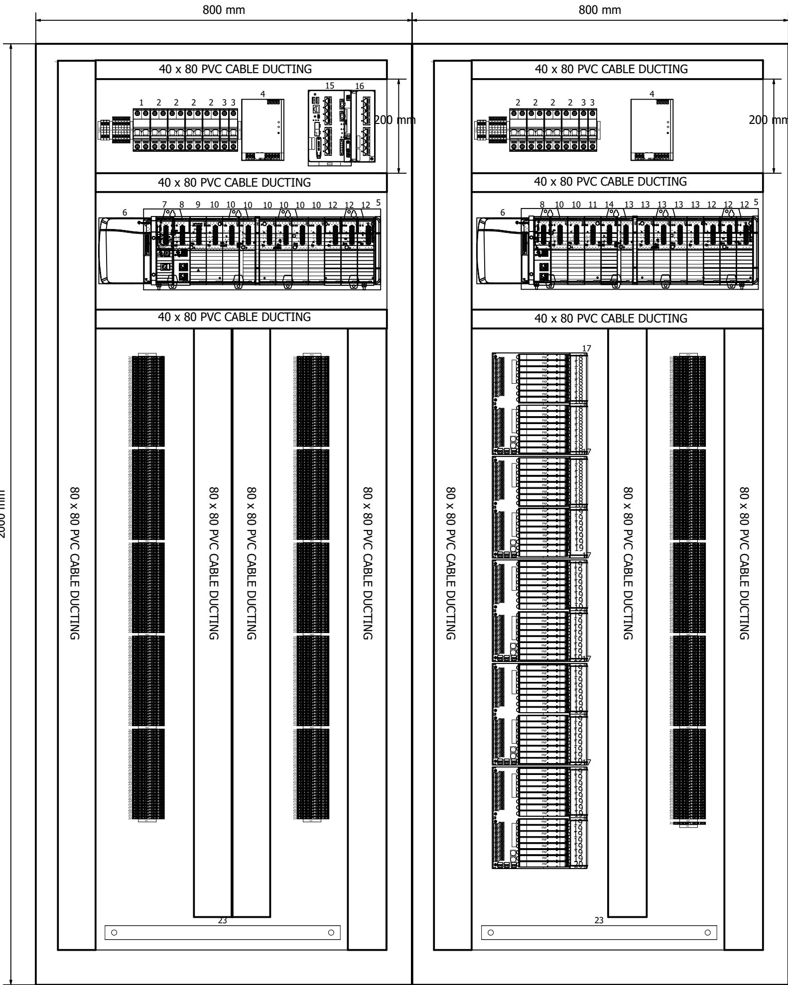
=CA1+MCP-M1 (FRONT)
