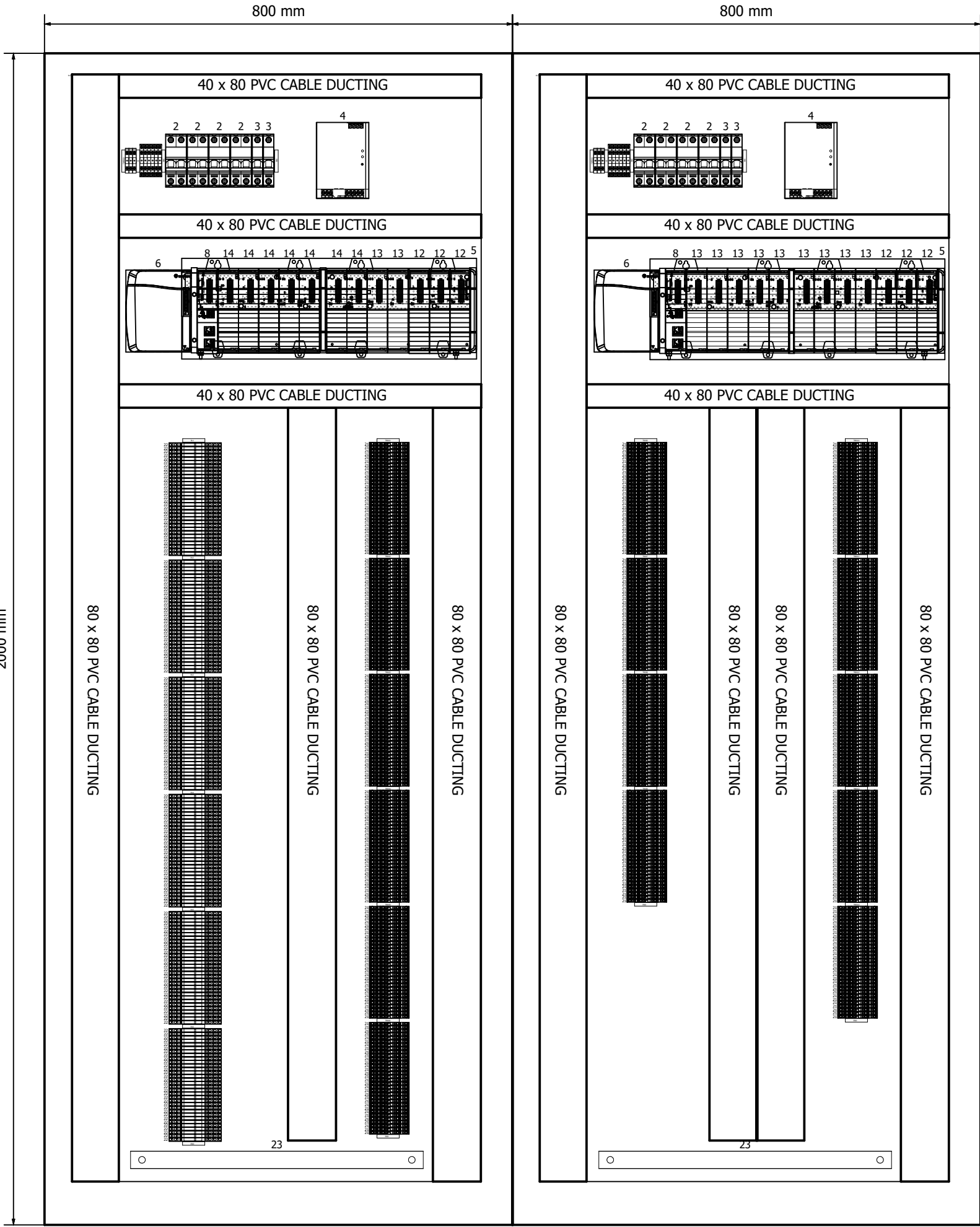
=CA1+MCP-M2 (REAR)
